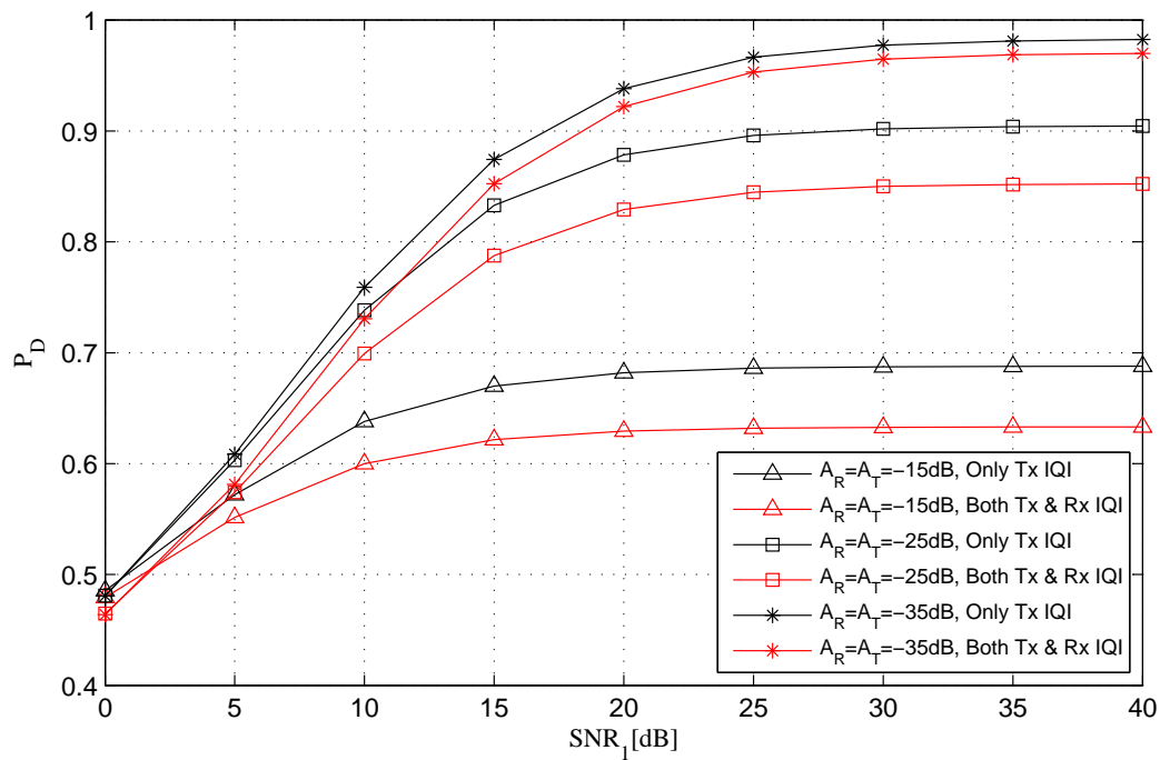
Fig. 5. The comparison of joint transmitter-receiver I/Q imbalance effect on the probability of detection with the case when I/Q imbalance exists only in transmitters for different values of IRRs. The IRR values are assumed to be identical in transmitters and receivers, i.e., A_T = A_R .
