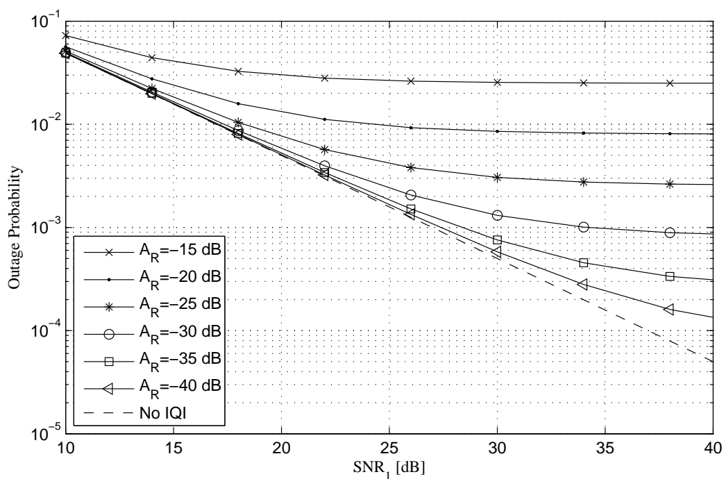
Fig. 6. The effect of I/Q imbalance on outage probability of primary system for different values of IRRs
